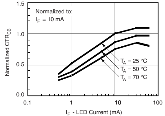
Fig. 6 - Normalized CTR_{cb}
